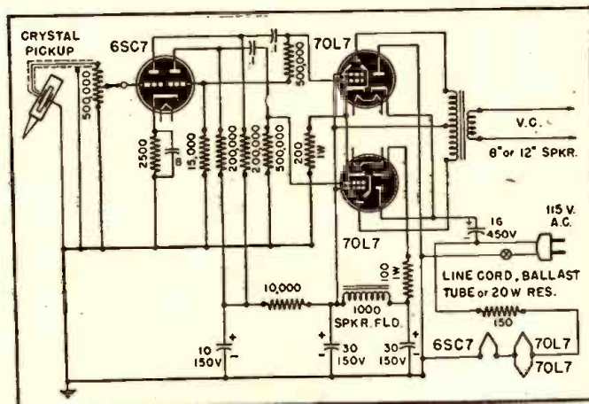
Fig. 1—An efficient high-fidelity amplifier for phonograph work.
