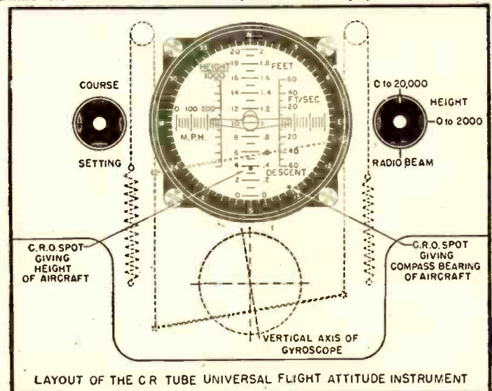
Fig. 3—A layout of the cathode-ray tube Universal Flight Attitude instrument. The electronically-traced airplane acts as its own indicator, giving information by its size and position on the screen.
